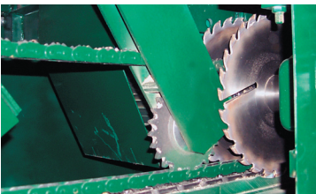
Each Model 1800 features two vertical edger blades at the infeed.
