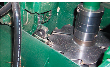
Finished boards are manufactured by the horizontal blades, positioned at the outfeed.
